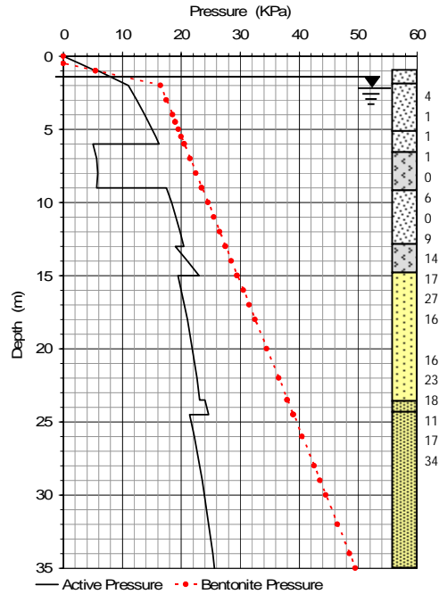
Figure 3: Bore stability assessment
