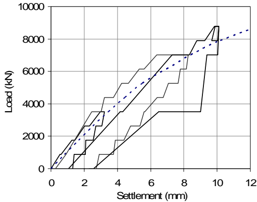
Figure 6: Pile load-settlement curve
