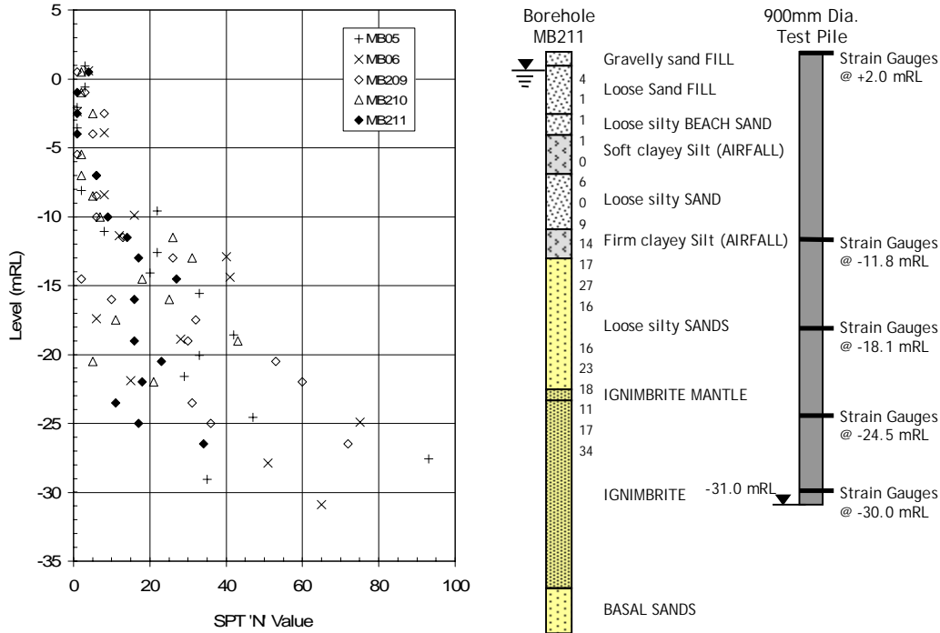
Figure 1: Geological profile near the test pile
