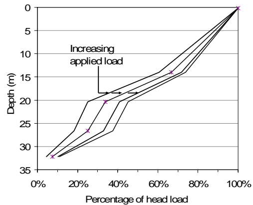
Figure 7: Load distribution along shaft
